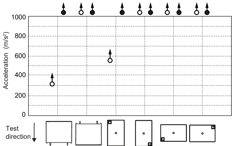
Shock resistance characteristics
