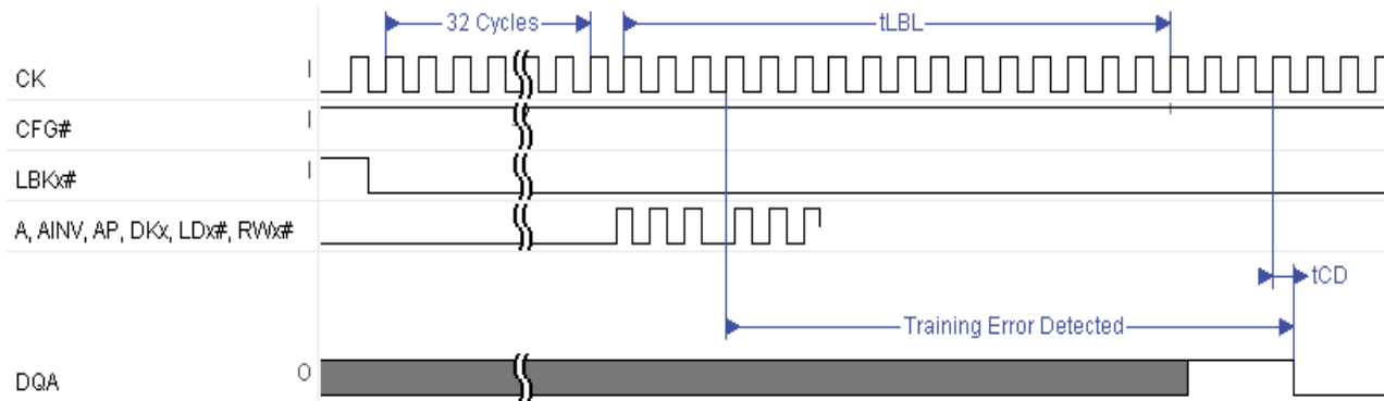
Figure 15. Loopback Timing
