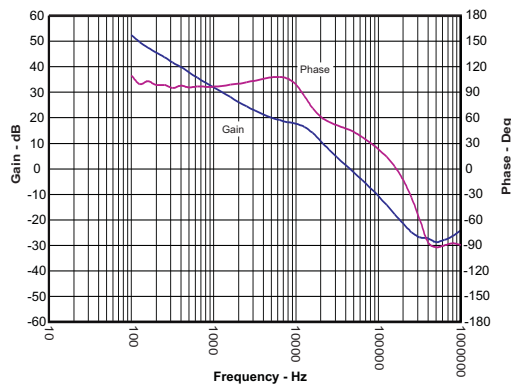
Figure 47. Closed-Loop Response
