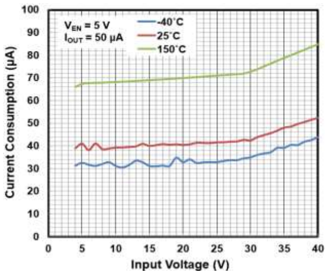
Figure 9. Current Consumption vs. Input Voltage
