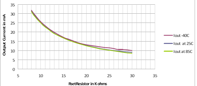
Output Current vs Rset Resistor
