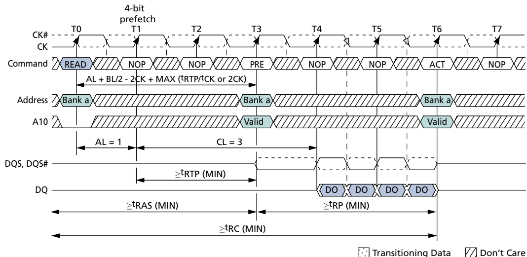
Figure 48: READ-to-PRECHARGE – BL = 4
