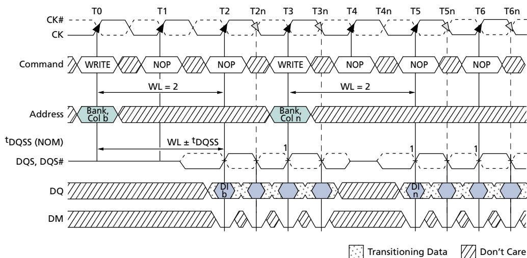
Figure 57: Nonconsecutive WRITE-to-WRITE
