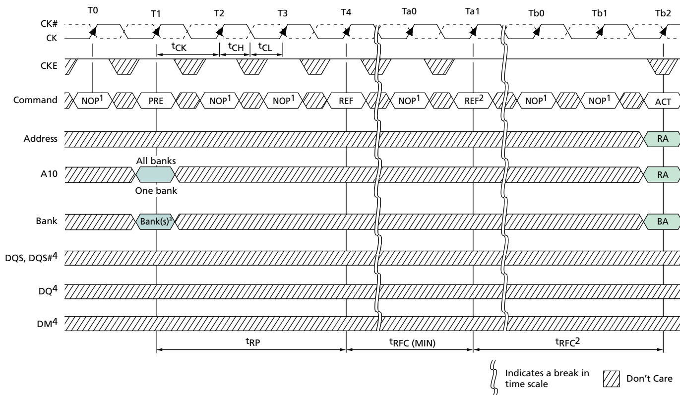
Figure 65: Refresh Mode
