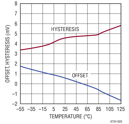
Input Offset and Hysteresis vs Temperature, V_{CC1} = V_{CC0} = 5.0V
