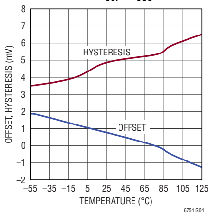
Input Offset and Hysteresis vs Temperature, V_{CC1} = V_{CC0} = 2.5V
