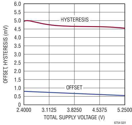
Input Offset and Hysteresis vs Supply Voltage, V_{CM} = 0.3V
