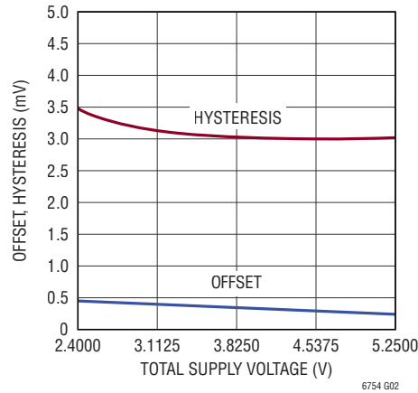
Input Offset and Hysteresis vs Supply Voltage, V_{CM} = V_{CC} - 0.3V
