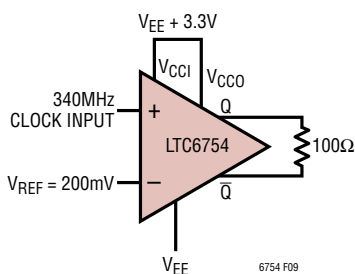
Figure 9. Corrupted Clock Recovery to LVDS Translator Circuit.
