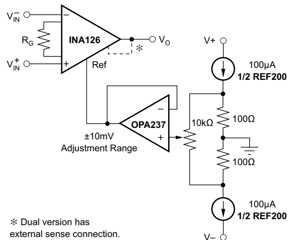
Figure 8-2. Optional Trimming of Output Offset Voltage
