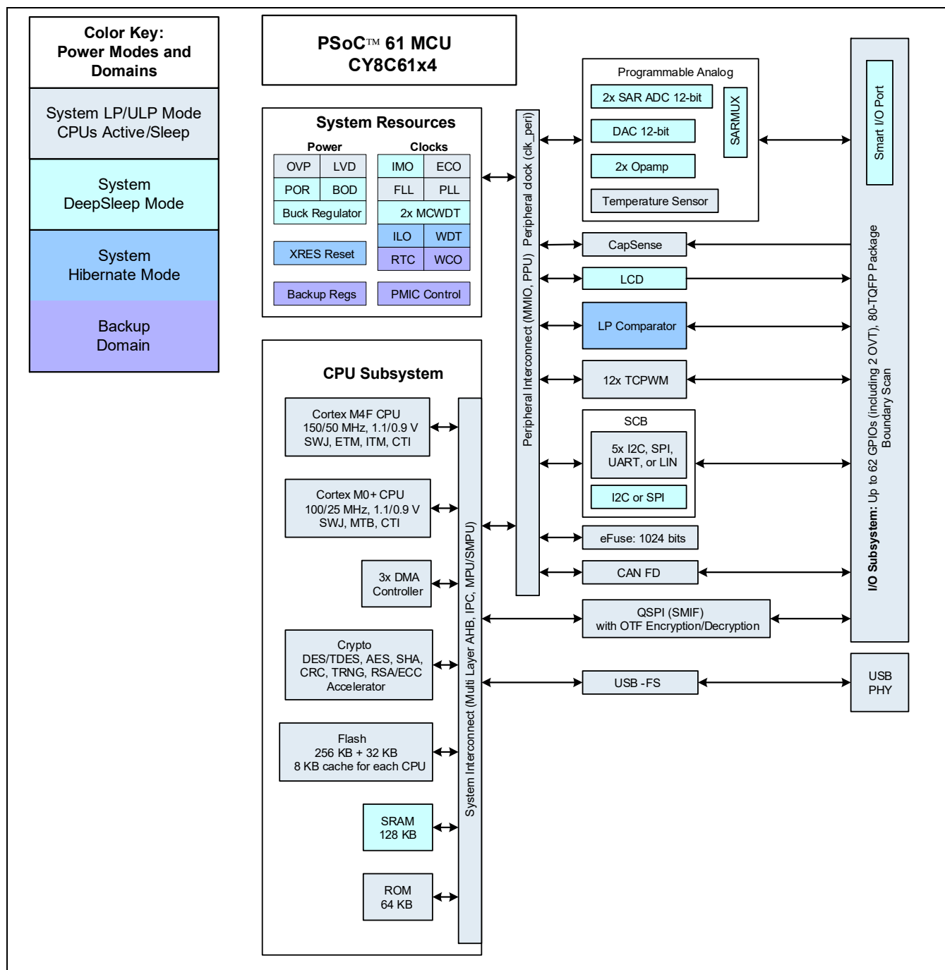
Figure 2 Block diagram
