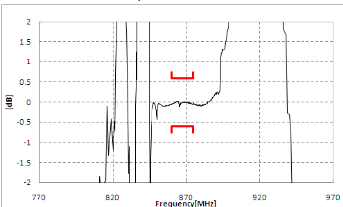
Amplitude Balance
