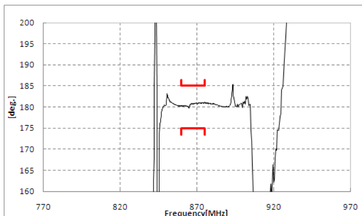
Phase Balance
