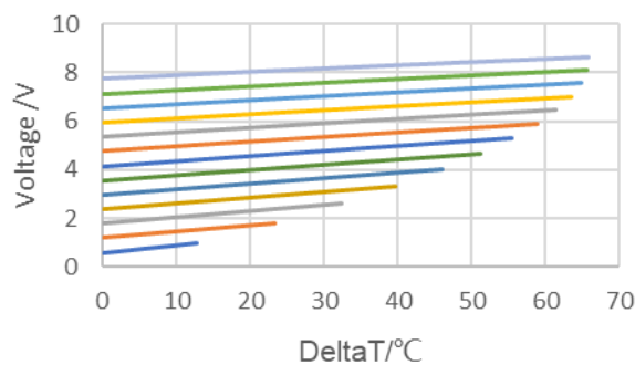
Performance Curves at T_h = 27^\circ\text{C}
