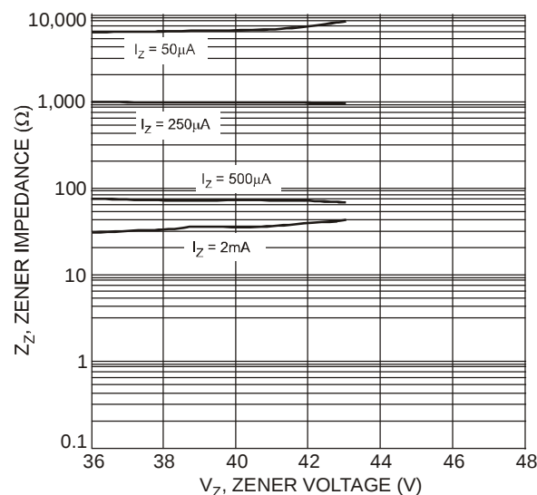
Fig. 15 Typical Zener Impedance Characteristics, DDZ36 - DDZ43
