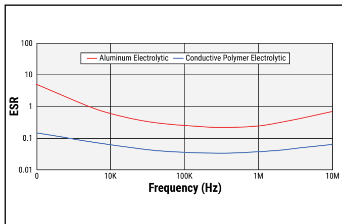
Stable ESR Values across Frequency
