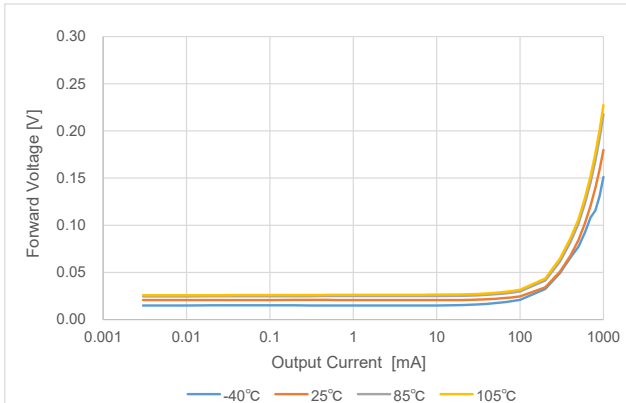
(6-1-2) Forward Voltage vs Output Current
