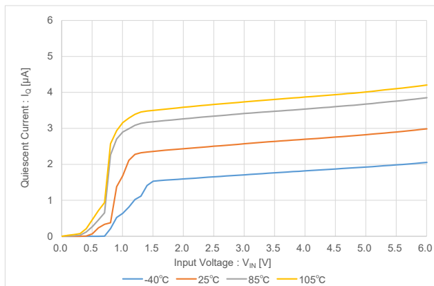
(2-1) Quiescent Current vs Input Voltage
