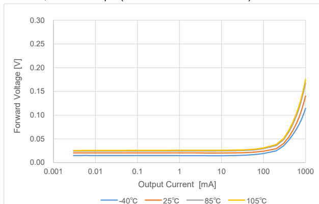
(6-1-3) Forward Voltage vs Output Current
