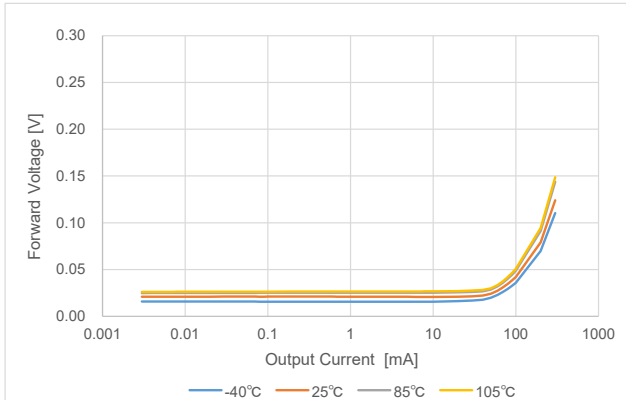
(6-1-1) Forward Voltage vs Output Current
