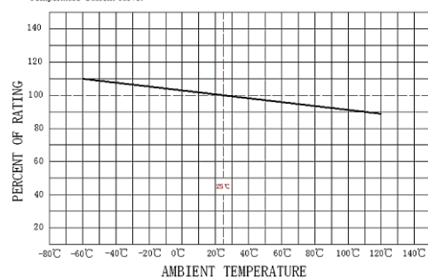
Temperature-Current curve:
