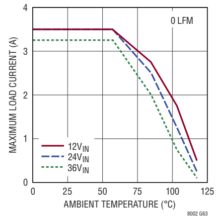
Derating, I-Grade, V_{OUT} = 2\text{V} , BIAS = 5V, DC2501A Demo Board
