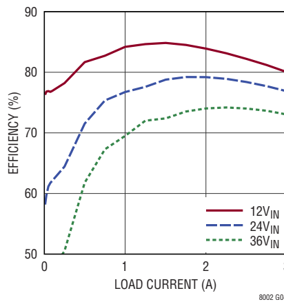
Efficiency, V_{OUT} = 1.8\text{V} , BIAS = 5V
