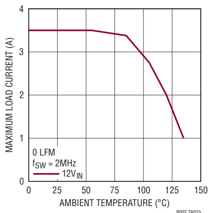
Derating, H-Grade, BIAS = 5V, DC2501A Demo Board
