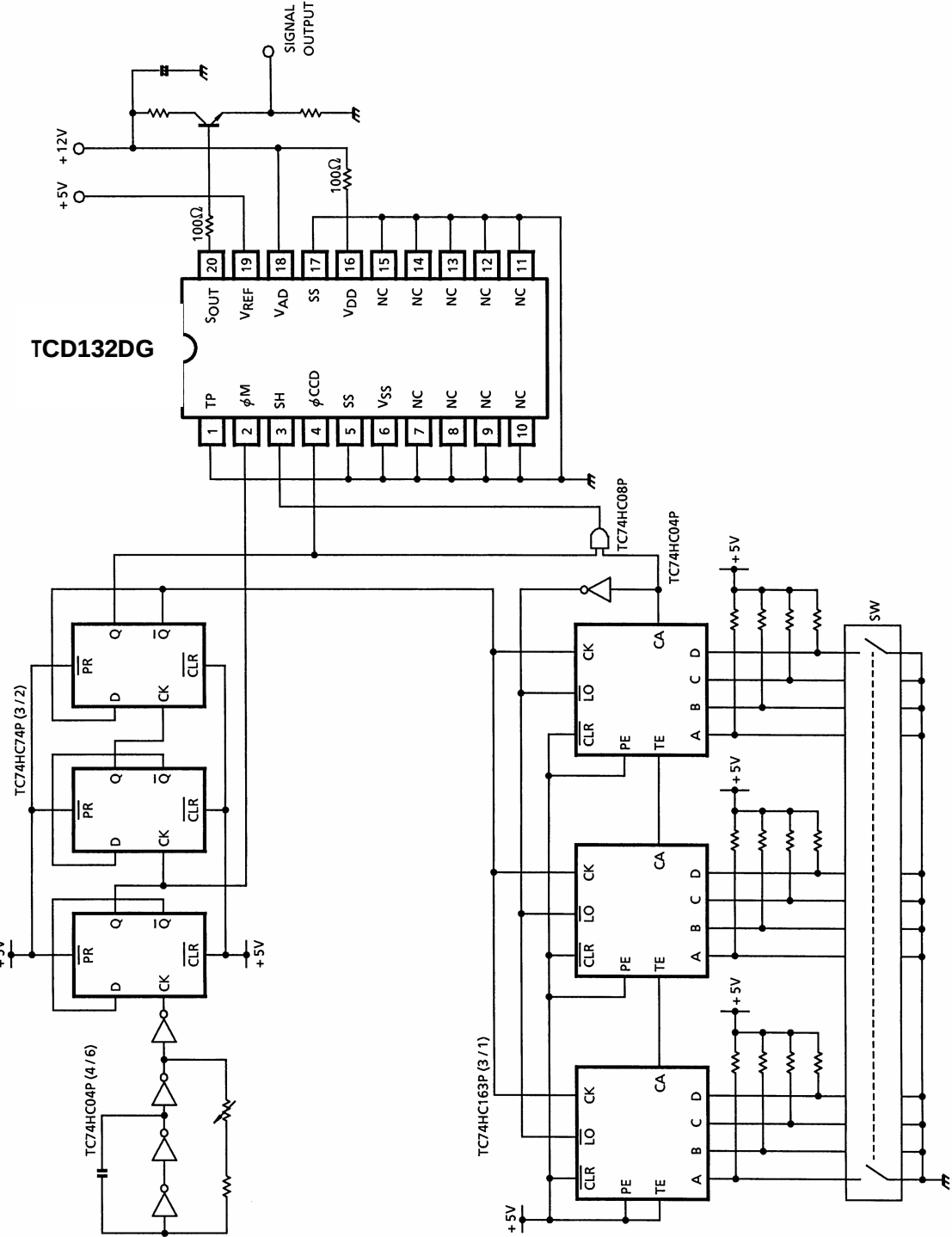
EXAMPLE OF OPERATING CIRCUIT
