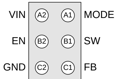
Figure 3. Bumps Facing Up
