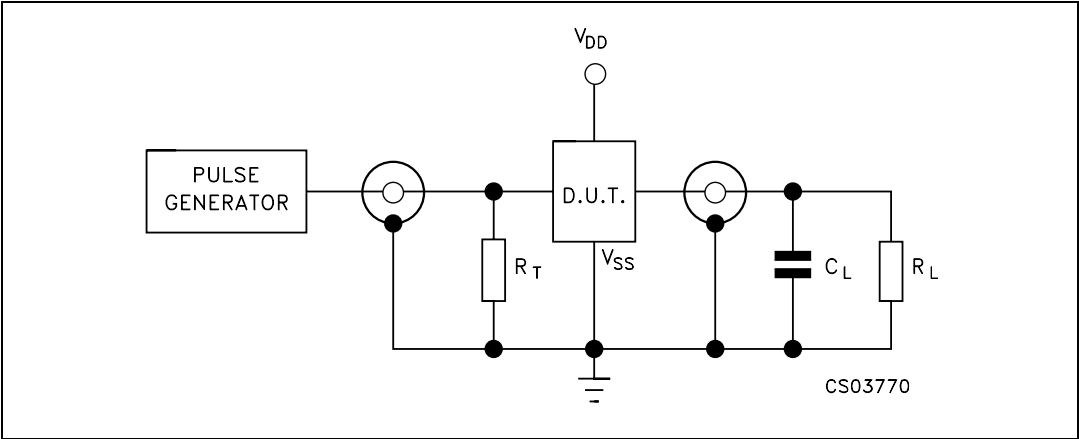
Figure 3. Test circuit
