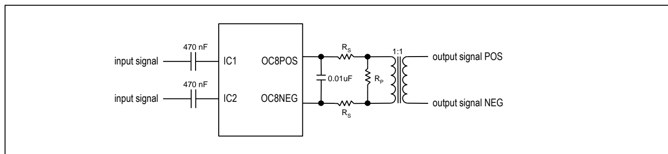
Figure 10-3. Recommended External Components for AMI Composite Clock Pins
