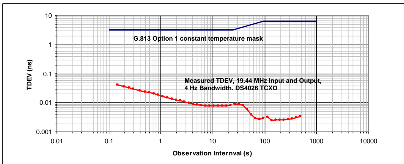
Figure 7-4. Typical TDEV for T0 DPLL Output
