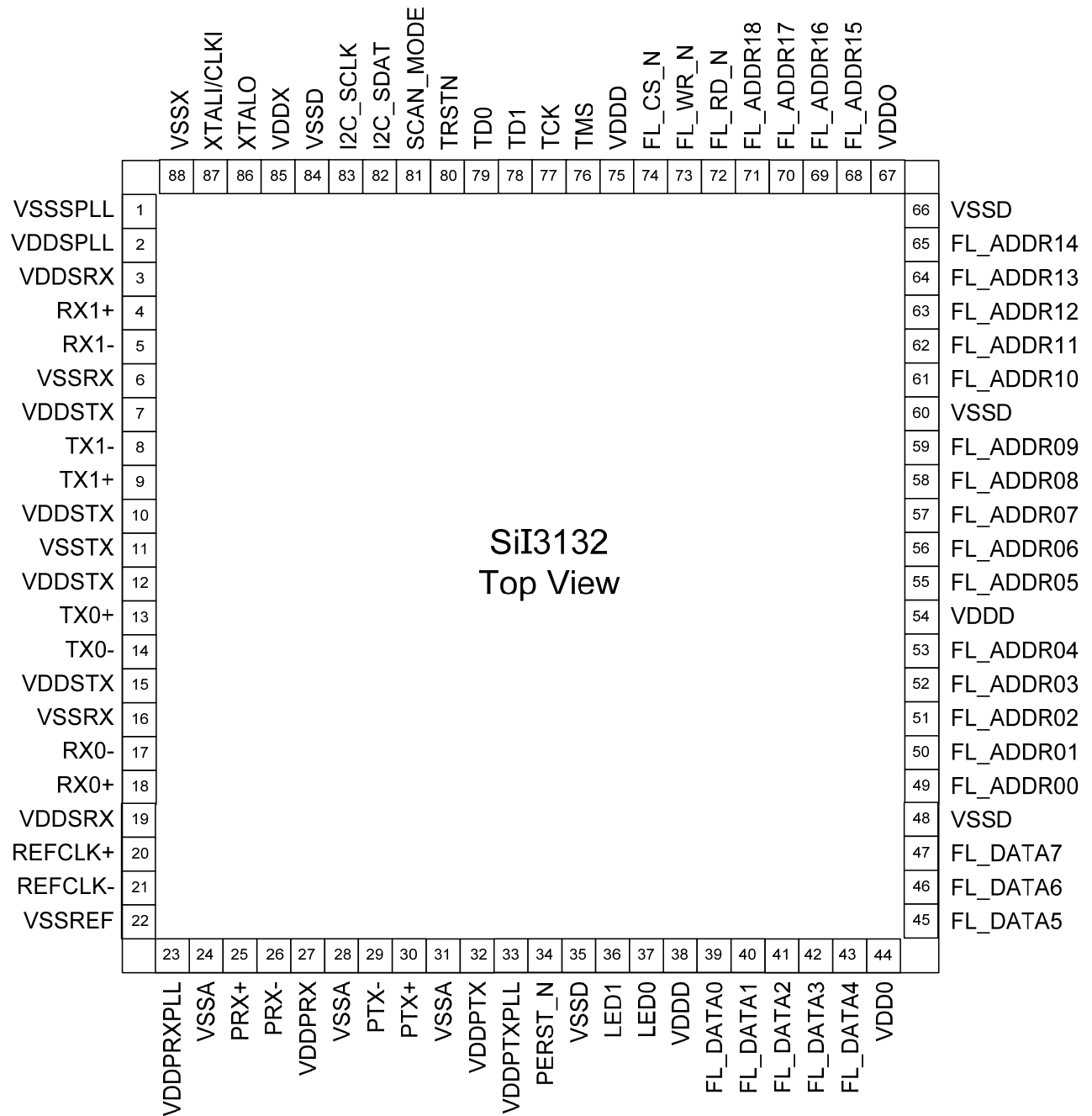
Figure 1. Pin Diagram (Top View)
