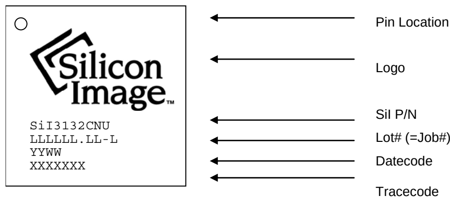
Figure 4. Marking Specification
