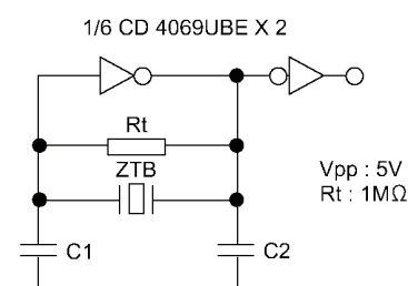
Figure 3) Test Circuit
