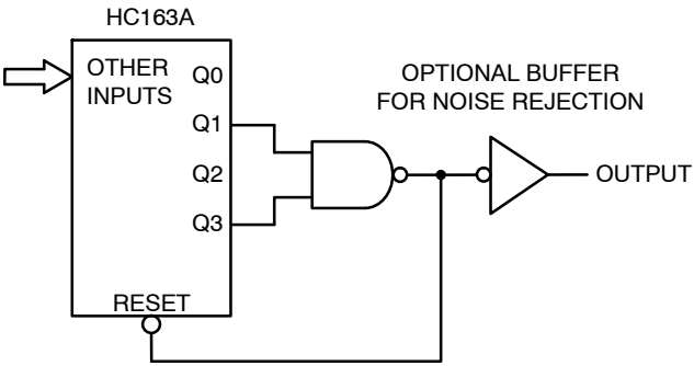
Figure 17. Modulo-11 Counter
