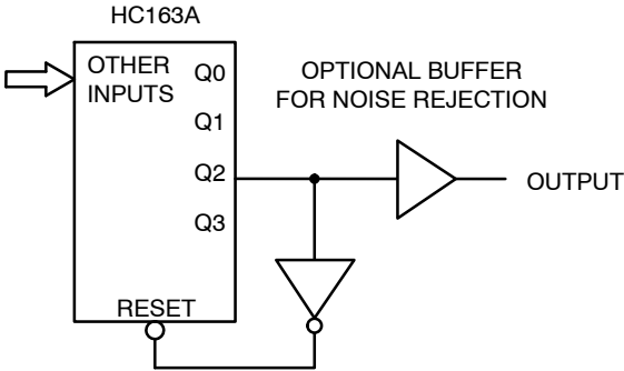
Figure 16. Modulo-5 Counter
