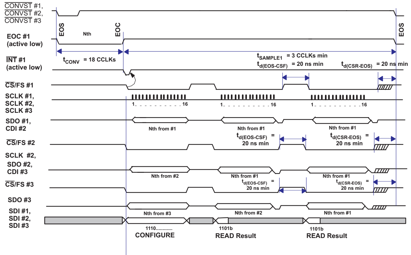
Figure 61. Simplified Cascade Mode Timing with Shared \overline{\text{CONVST}} and Discrete \overline{\text{CS}}
