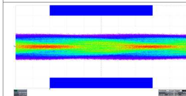
Figure 6. No Re-Driver, Trace Length = 24"+3m Cable
