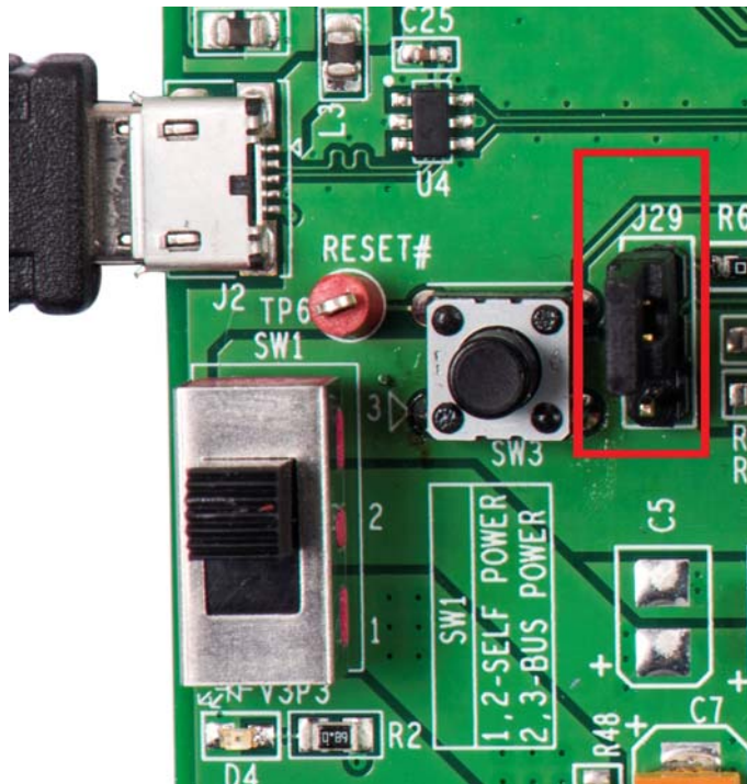
Figure 3-37. VBUS Selection
