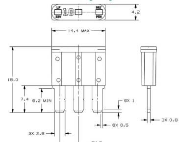
Dimensions [mm]
