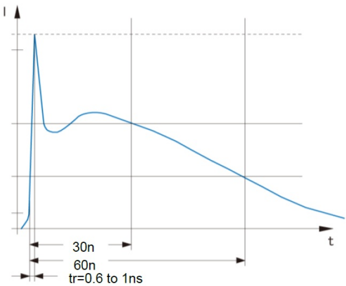
IEC61000-4-2 Waveform
