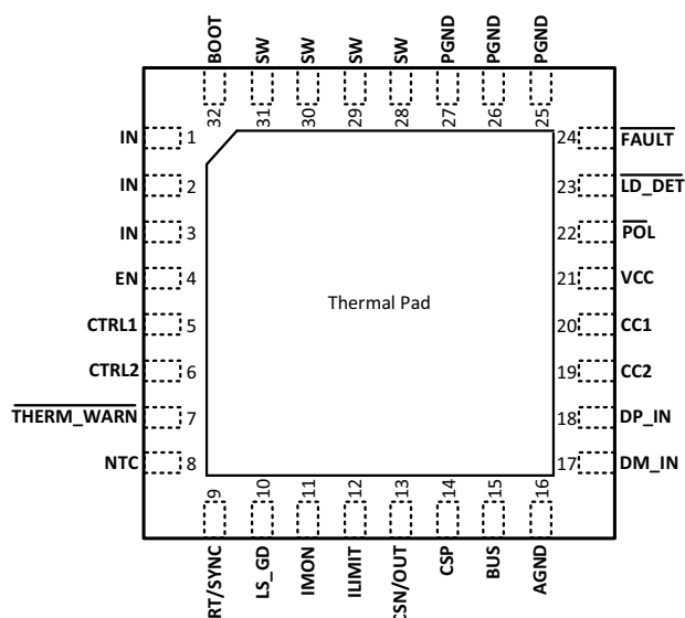
Figure 7-4. TPS25831QCWRHBRQ1 Package 32-Pin (VQFN) Top View (2)
