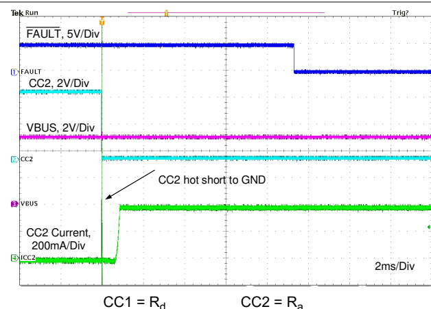
Figure 11-30. CC2 Hot Short to GND
