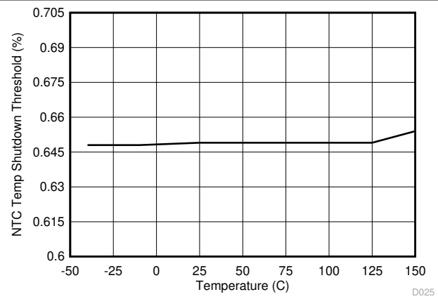
Figure 8-28. NTC Temperature Shutdown Threshold (TPS25831-Q1)
