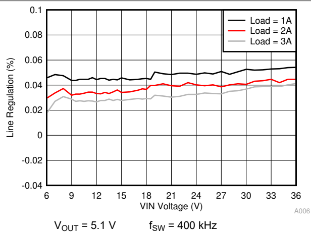
Figure 11-7. Line Regulation
