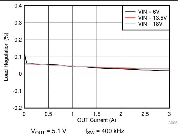
Figure 11-6. Load Regulation
