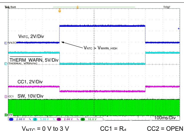
Figure 11-37. Thermal Sensing With NTC Behavior
