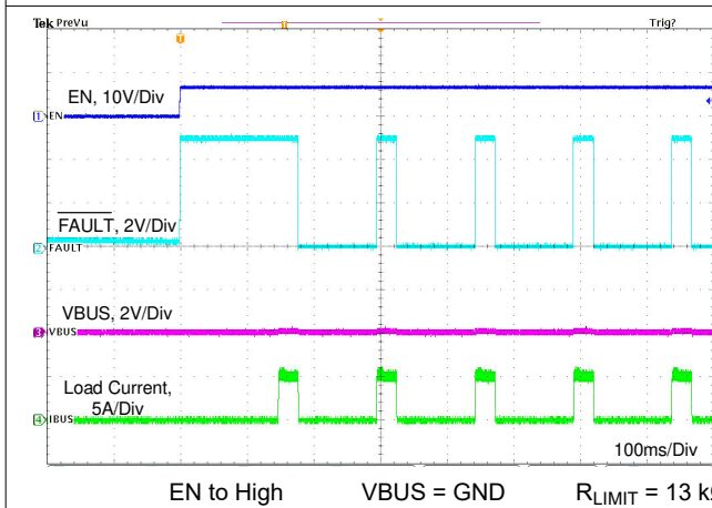
Figure 11-22. Enable Into Short Without External FET
