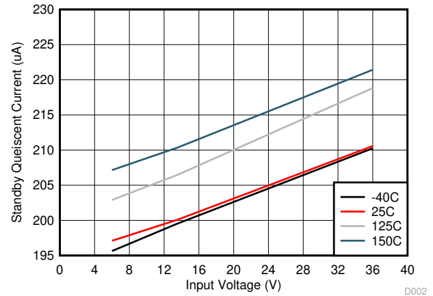
Figure 8-2. Standby Quiescent Current
