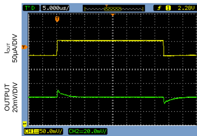
Figure 2: TS6001 Transient Load Regulation Response, C_{LOAD} = 1000pF
