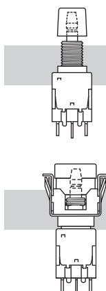
Snap-in Mount
