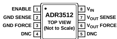
Figure 2. Pin Configuration
