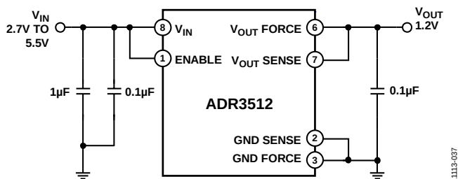
Figure 37. Basic Reference Connection
