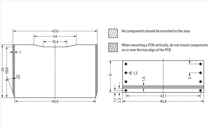
Empty component plug housing, type 11
