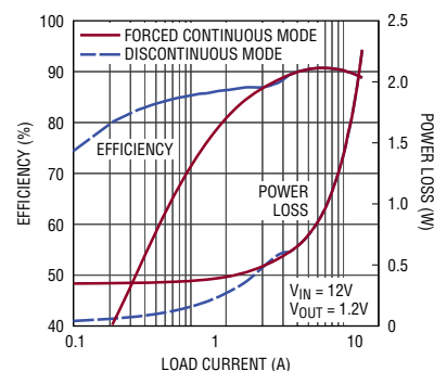
Efficiency/Power Loss
