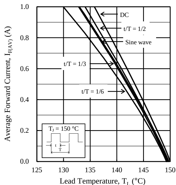
Figure 3. Typical Characteristics: I_{F(AV)} vs. T_L ( V_R = 100 V)
