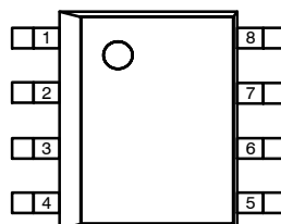
Figure 3. SOIC-8 (Top View)
