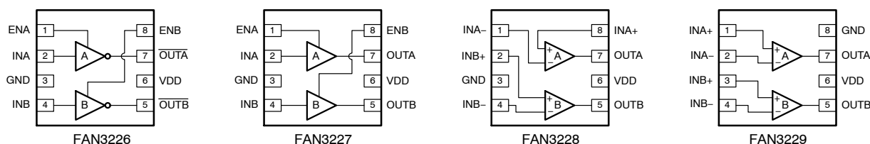
Figure 1. Pin Configurations
