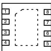
Figure 2. 3x3 mm MLP-8 (Top View)
