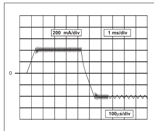
Figure 4. Motor current ( I_M ), Vertical : 200 mA/div, Horizontal: 1 ms/div, expanded part 100 μs/div.
