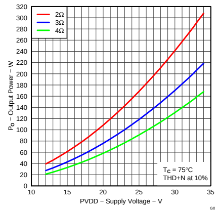
Figure 21. Output Power vs Supply Voltage
