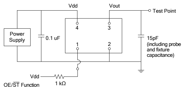
Figure 1. Test Circuit
