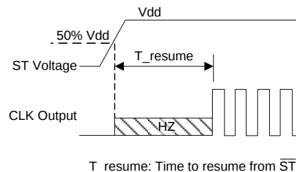
Figure 4. Standby Resume Timing (ST Mode Only)
