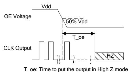
Figure 6. OE Disable Timing (OE Mode Only)
