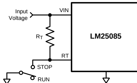
Figure 22. Shutdown Implementation
