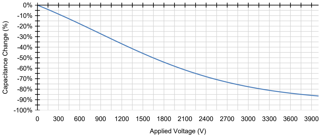
VCC Characterization
