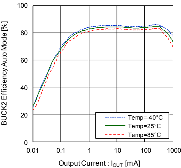
Figure 29. Efficiency vs Output Current ("BUCK2 Efficiency Auto Mode", V_{BAT}=3.6V , V_{OSW2}=1.3V )
