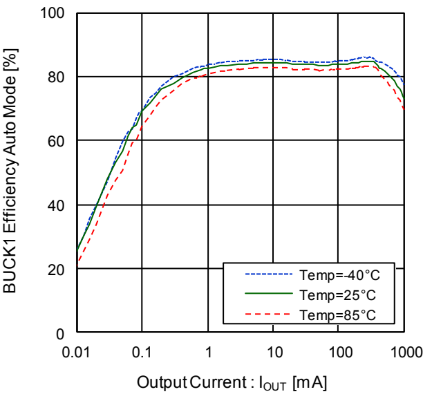
Figure 27. Efficiency vs Output Current ("BUCK1 Efficiency Auto Mode", V_{BAT}=3.6V , V_{OSW1}=1.3V )
