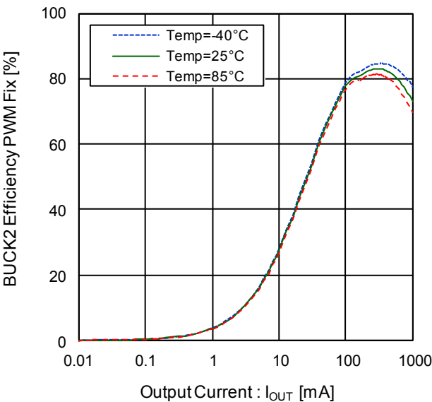
Figure 30. Efficiency vs Output Current ("BUCK2 Efficiency PWM Mode", V_{BAT}=3.6V , V_{OSW2}=1.3V )
