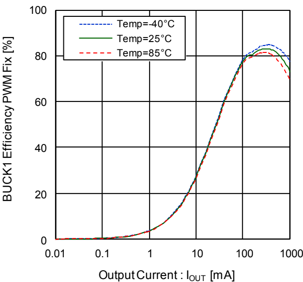
Figure 28. Efficiency vs Output Current ("BUCK1 Efficiency PWM Mode", V_{BAT}=3.6V , V_{OSW1}=1.3V )
