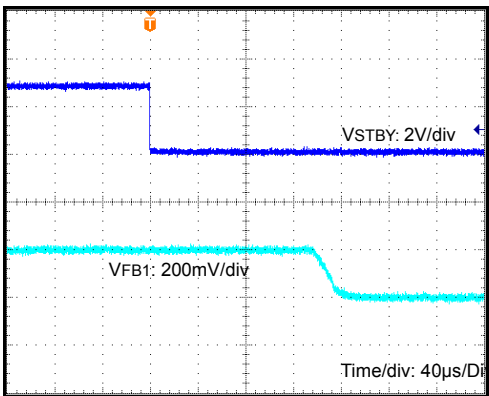
Figure 45. BUCK1 DVS Fall Time (V BAT =3.6V C L =10µF I OUT =0A Ramp Rate=10mV/µs, BUCK1_MODE [02h:15h] PWM Mode)
