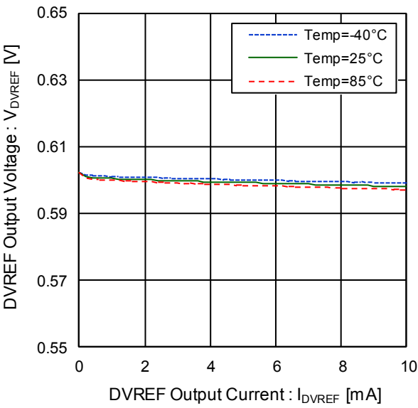
Figure 43. DVREF Output Voltage vs DVREF Output Current (V BAT =3.6V, V SYS =V IN =V INL1,2 )
