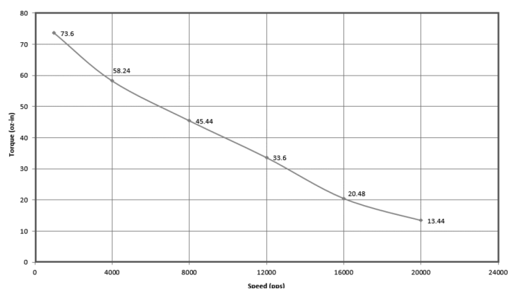
Same Sky P/N NEMA23-17-01PD-AMT112S Lin Engineering P/N WD-5718X-01P (1.8 Step Motor) 24 Vdc, 2.8 Amp/Phase, 1B463, 1/2 Stepping
