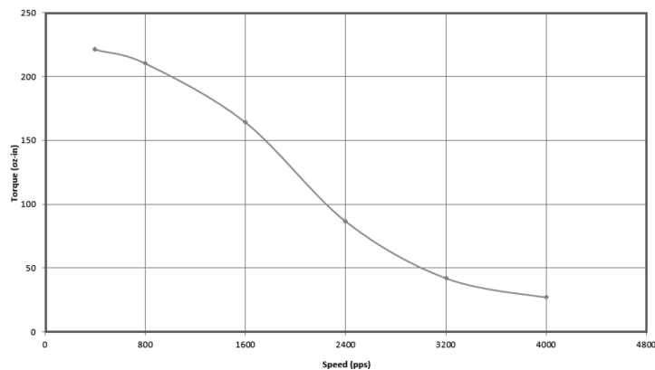
Same Sky P/N NEMA23-31-01PD-AMT112S Lin Engineering P/N WD-5718L-01P (1.8 Step Motor) 24 Vdc, 2.8 Amp/Phase, IB463, 1/2 Stepping
