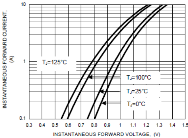
FIG.3-TYPICAL FORWARD CHARACTERISTICS
