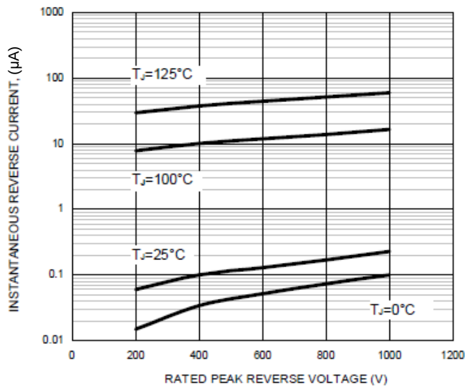
FIG.5-TYPICAL REVERSE CHARACTERISTICS
