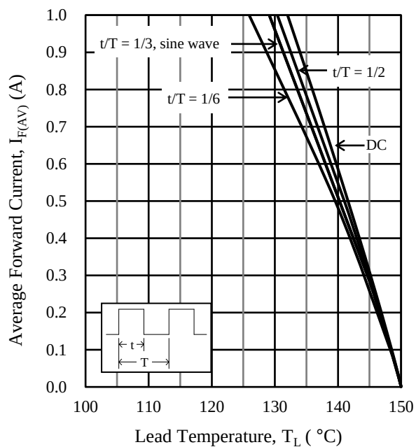
Figure 9. SARS05 I_{F(AV)} vs. T_L ( T_J = 150 °C, V_R = 0 V)
