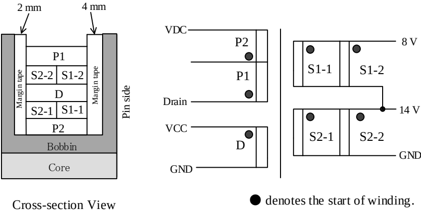
Figure 24. Winding Structure
