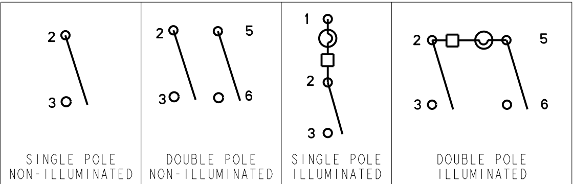
CIRCUIT DIAGRAMS 5
