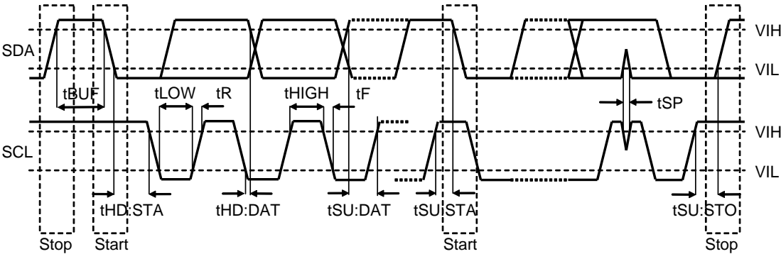
Figure 13. I²C Bus Timing
