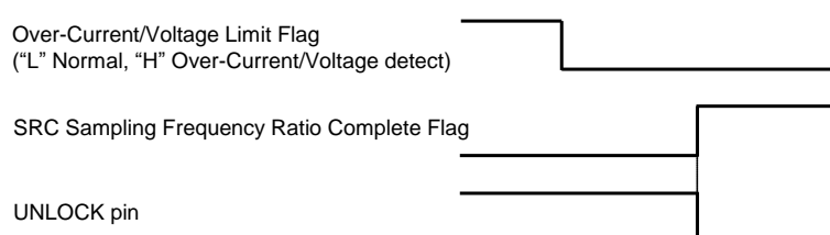
Figure 38. Internal Flags and UNLOCK pin Output
