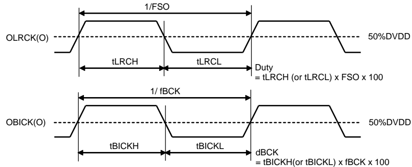
Figure 7. OLRCK, OBICK, Clock Timing (Slave Mode)
