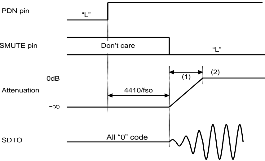
Note: SDTO is identified as SDTO1, SDTO2 and SDTO3. (1) The output data is attenuated by -\infty during the soft mute cycle (Table 9) (2) When it is 0dB by a soft mute release after 4410/FSO, it is able to mute or release the mute by the soft mute cycle in Table 9. Figure 33. Soft Mute Function (Semi-Auto Mode)
