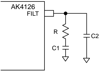
Figure 3. AK4126
