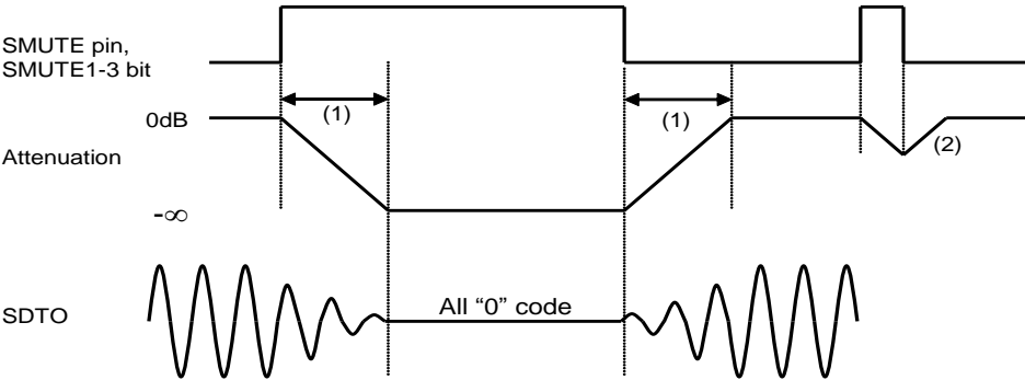
Note: SDTO is identified as SDTO1, SDTO2 and SDTO3. (1) The soft mute cycle is selected by SMT1-0 pins. (Table 9) The output data is attenuated by -\infty during the soft mute cycle. (2) If the soft mute is cancelled before attenuating to -\infty , the attenuation is discontinued and returned to 0dB by the same clock cycles. Figure 32. Soft Mute Function (Manual Mode) 2. Semi-Auto Mode
