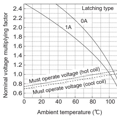
Operating range
