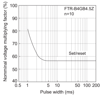
Pulse characteristics
