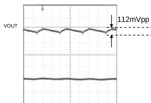
Figure 27. Output noise
