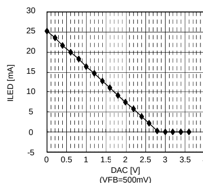
Figure 19. DAC adjustment
