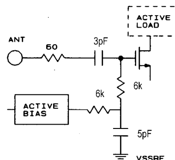
Figure 1 ANT Pin
