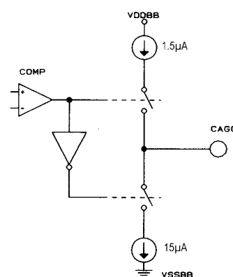
Figure 3 CAGC Pin
