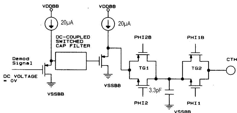
Figure 2 CTH Pin
