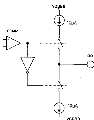
Figure 4 DO Pin
